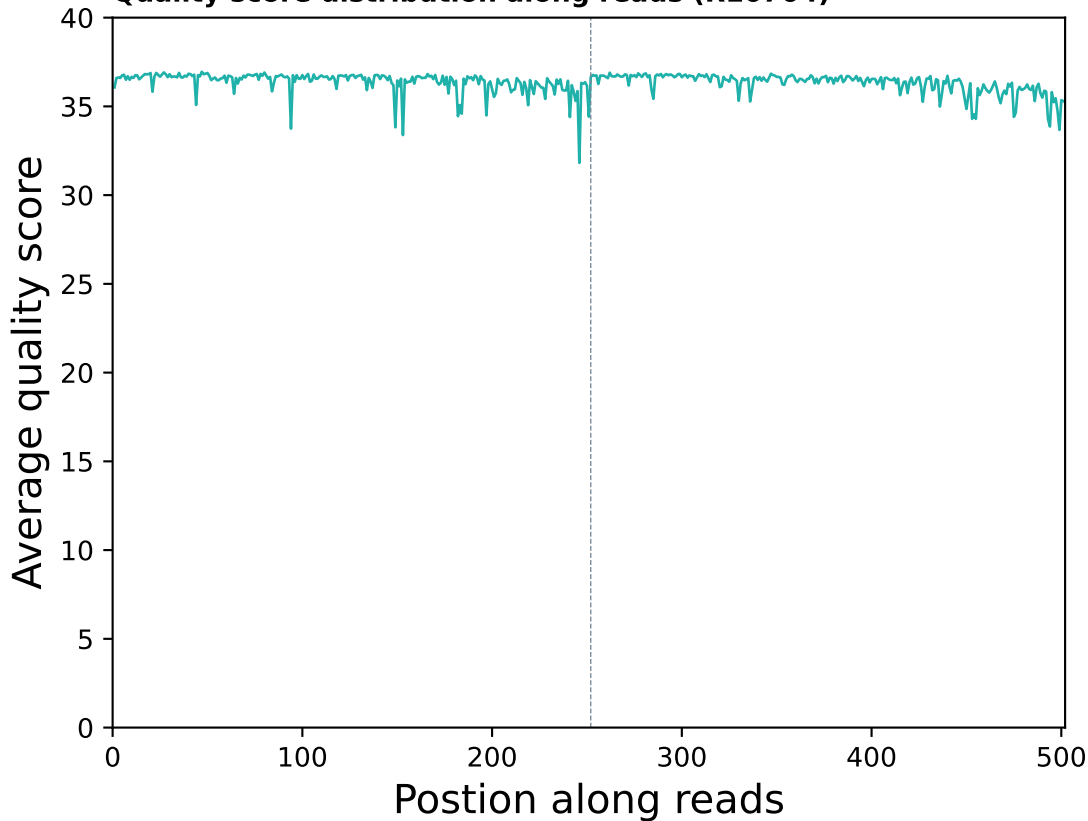
Quality score distribution along reads (R10704)
